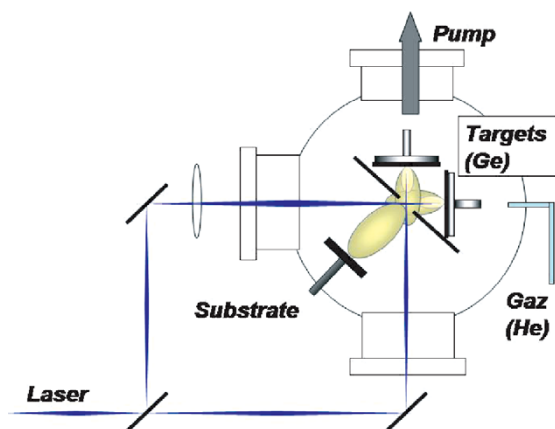
Figure 1. Schematic diagram of the CBPLD set-up.
